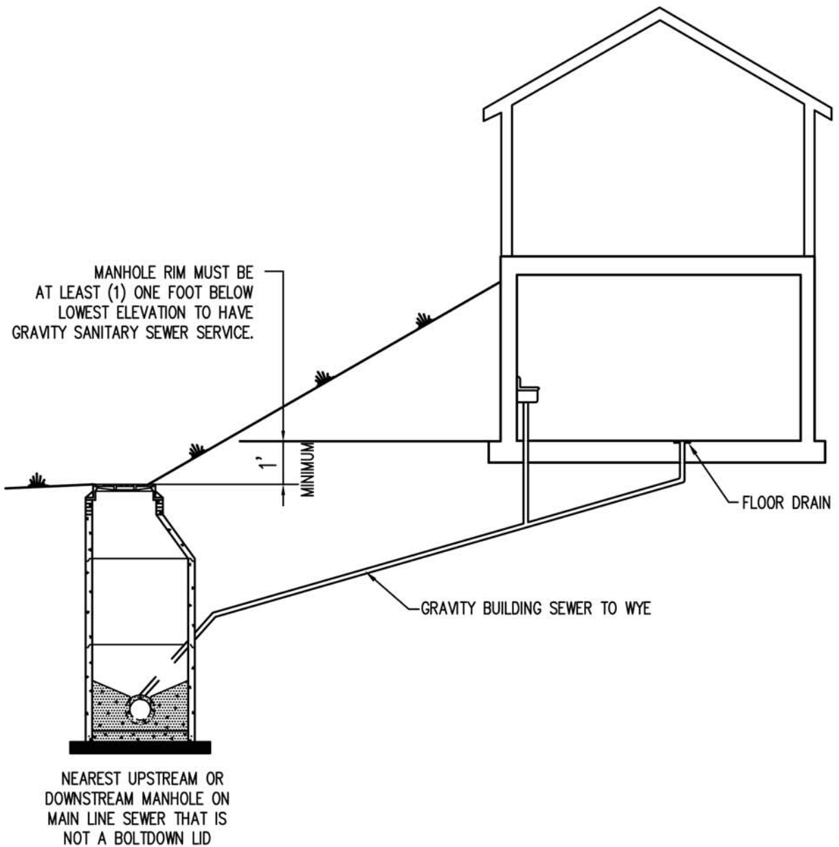
ACCEPTED DESIGN OF SANITARY SEWER BUILDING CONNECTION
